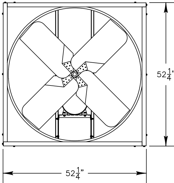
DISCHARGE VIEW
